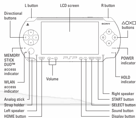
PSP® (PlayStation®Portable) system configuration
